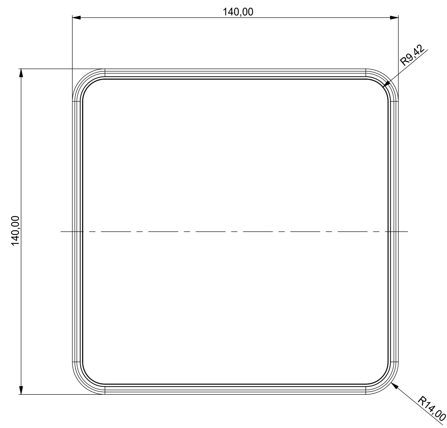
Ansicht "Z" View "Z"
