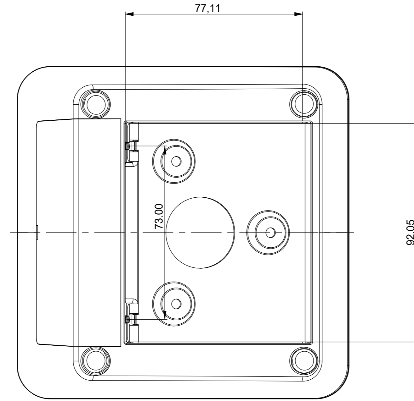
Ansicht "Y" View "Y"
