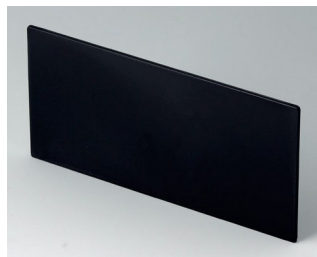
B6143221 Front panel PPO (UL 94 V-0) black RAL 9005 139,3x67,5x2,2mm
