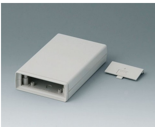
A9408336 BOITIER COQUILLES V 155, Vers. IV ABS (UL 94 HB) gris blanc RAL 9002 95x158x33mm
